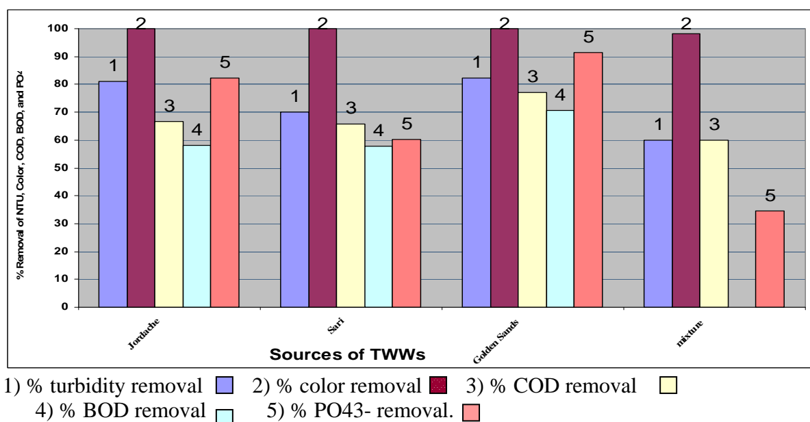
Figure (8): Treatment of TWWs using optimum dose of Azraq bentonite after (Al Sghireen, 2006).
