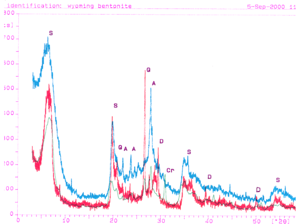
Figure (3): XRD trace of Q'a Al Azraq bentonite and Wyoming bentonite ( Nawasreh, 2001).
