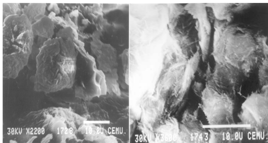
Figure (4): SEM micrographs of bentonite samples from Q'a Al Azraq (Nawasreh, 2001).
